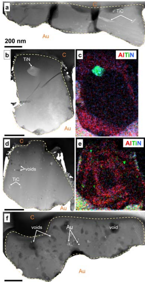
Figure 1. STEM HAADF images and EDS X-ray maps of presolar SiC grains: (a) MS G312, (b–c) MS G620, (d–e) MS G619, and (f) X G674. The SiC grains are outlined.
