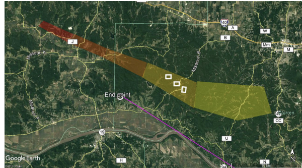
Figure 2: Strewn field calculation. Pink line is bolide path; white rectangles indicate search area. Red is the predicted area for \sim kilogram meteorites, yellow is the predicted area for sub-gram meteorites.
